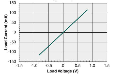
Typical Load Current vs. Load Voltage ( I_F=1\text{mA} )
