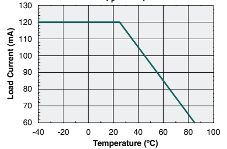
Maximum Load Current vs. Temperature ( I_F=2\text{mA} )
