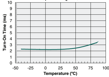
Typical Turn-On Time vs. Temperature ( I_F=5mA, I_L=1A )
