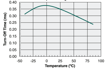
Typical Turn-Off Time vs. Temperature ( I_F=5mA, I_L=1A )
