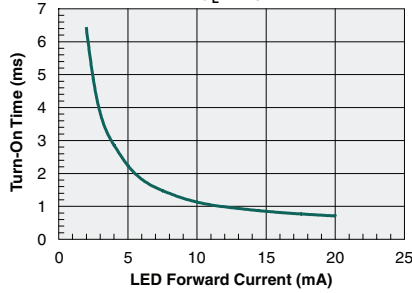
Typical Turn-On Time vs. LED Forward Current ( I_L=1A )
