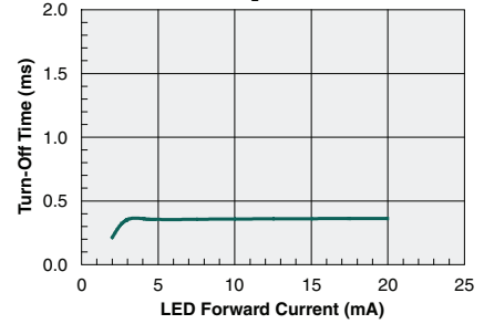
Typical Turn-Off Time vs. LED Forward Current ( I_L=1A )
