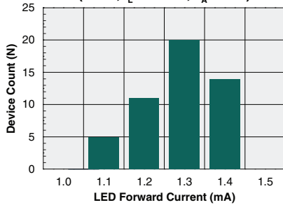
Typical I F for Switch Operation (N=50, I L =500mA, T A =25°C)
