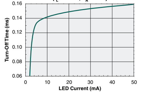
Typical Turn-Off Time vs. LED Forward Current ( I_L=75mA , T_A=25^\circ C )
