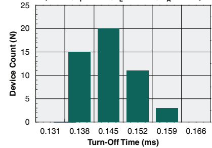
Typical Turn-Off Time (N=50, I F =5mA, I L =75mA, T A =25°C)
