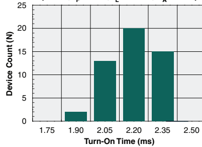
Typical Turn-On Time (N=50, I F =5mA, I L =75mA, T A =25°C)
