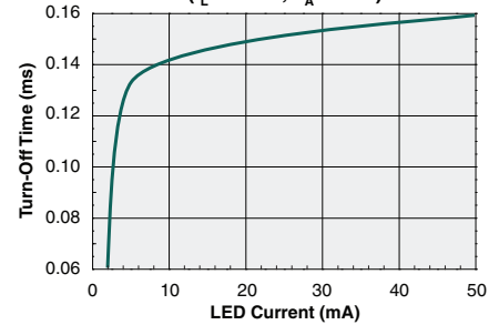
Typical Turn-Off Time vs. LED Forward Current (I L =75mA, T A =25°C)
