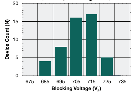
Typical Blocking Voltage Distribution (N=50, I F =0mA, T A =25°C)
