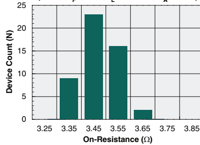
Typical On-Resistance Distribution (N=50, I F =5mA, I L =500mA, T A =25°C)
