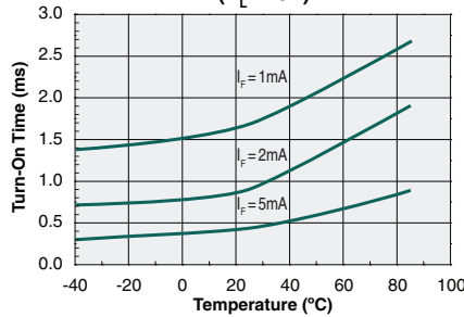
Typical Turn-On Time vs. Ambient Temperature ( V_L=10V )
