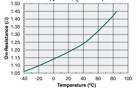
Typical On-Resistance vs. Temperature ( I_F=0\text{mA} , I_L=200\text{mA} )
