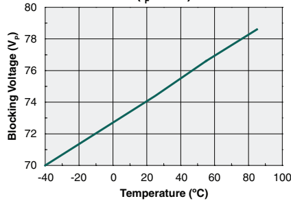
Typical Blocking Voltage vs. Temperature ( I_F=4\text{mA} )
