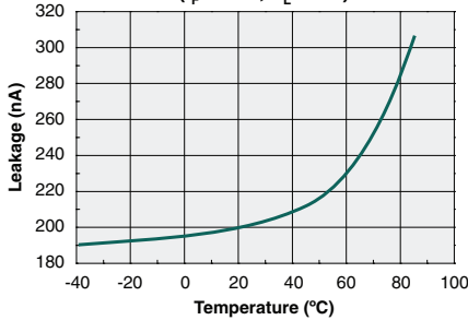
Typical Leakage Current vs. Temperature ( I_F=4\text{mA} , V_L=60\text{V} )
