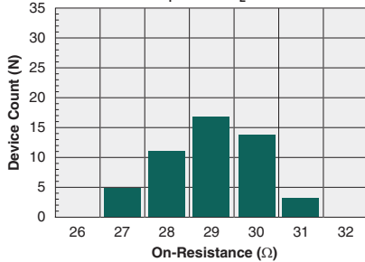
Typical On-Resistance Distribution (N=50, I F =2mA, I L =100mA)
