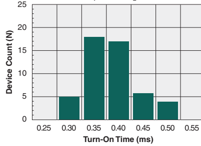
Typical Turn-On Time (N=50, I F =5mA, I L =150mA)
