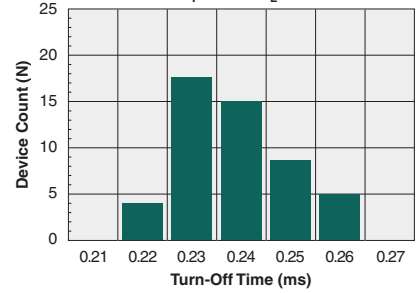
Typical Turn-Off Time (N=50, I F =5mA, I L =150mA)
