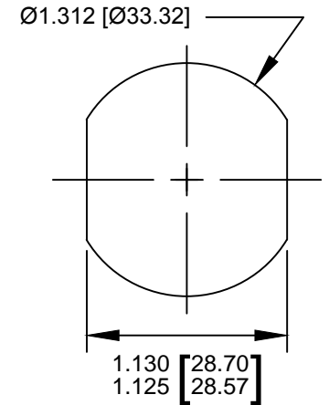
TYPICAL PANEL CUTOUT
