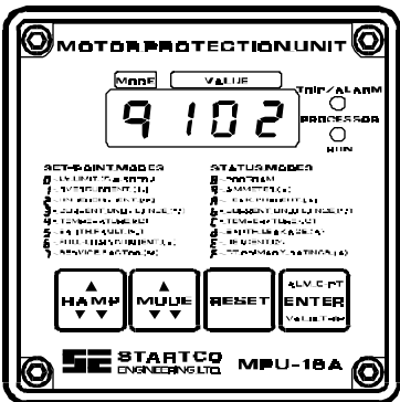
1-32 MPU-16A's
